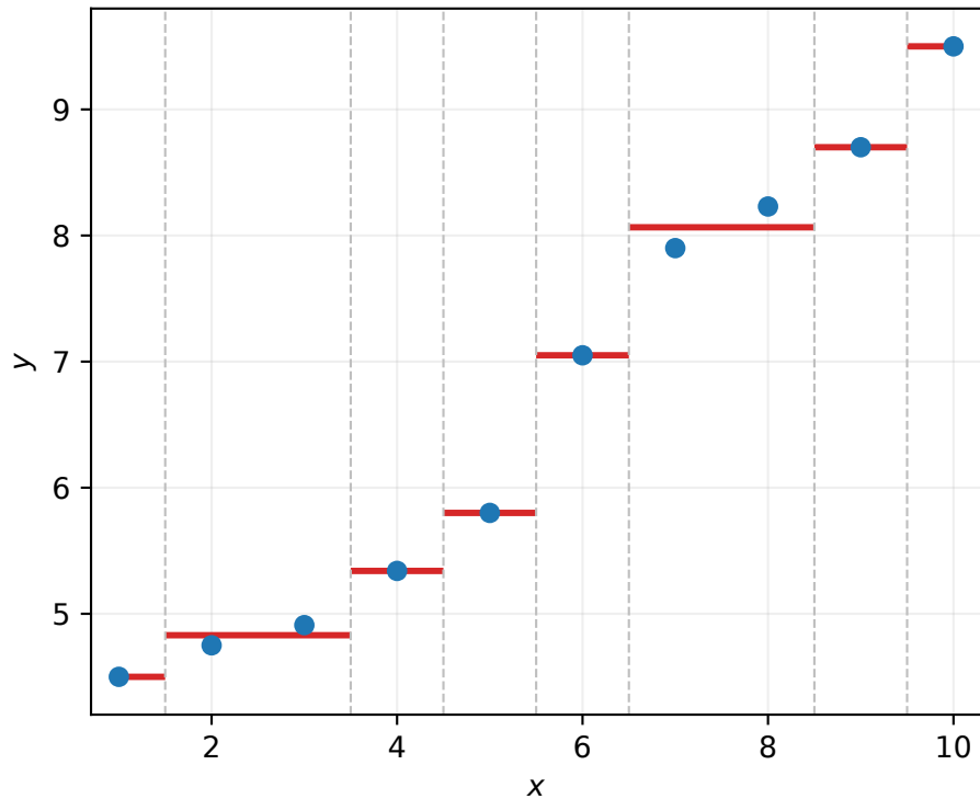
Piecewise constant prediction
