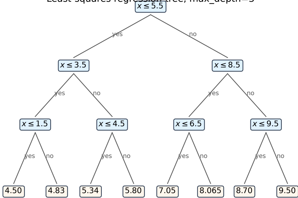
Least-squares regression tree, max_depth=3
